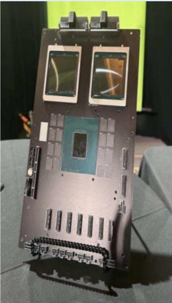
图：GB200 SuperChip
